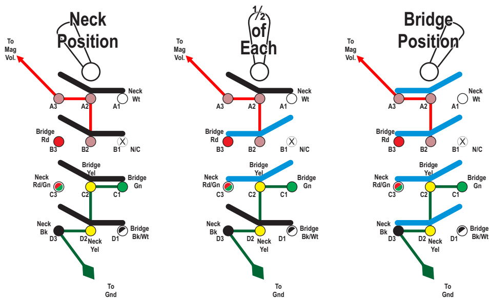
Switch Logic Table ( After-market "B" Logic )
