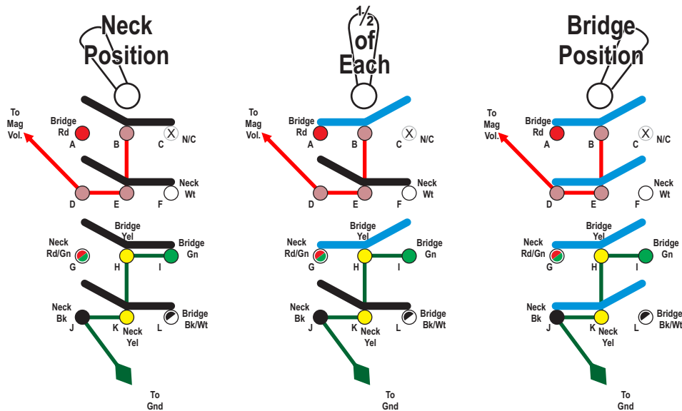
Switch Logic Table ( Stock OEM Switch )
